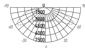
PSL 02 100W
