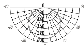
PBH-PC7-RSS 12W
