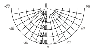
PBH-PC8-RA 12W
