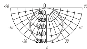
PWP-C3 40W
