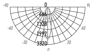
PWL-200110/30D 1X9W
