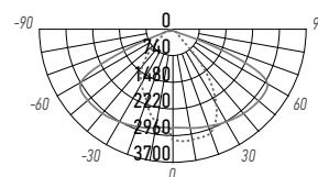
PSL 03 70W
