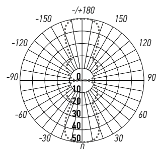
PWL-12080/40D 2X4W
