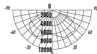
PSL 05-2 200W
