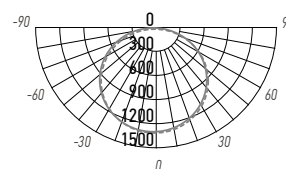
PP0-06 50W
