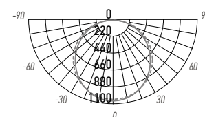
PWP-C4 36W
