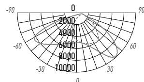
PSL 08 150W 140/70°
