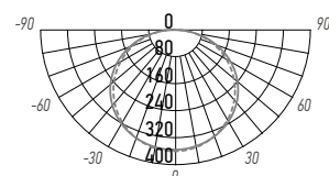
PBH-PC7 12W
